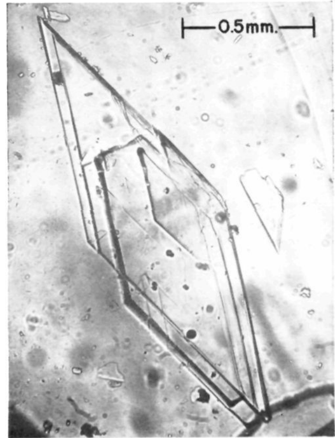
Fig. 2.—Human serum albumins crystallized from water saturated with decanol; \Gamma/2 < 0.001 ; pH 4.9; 0^\circ .
