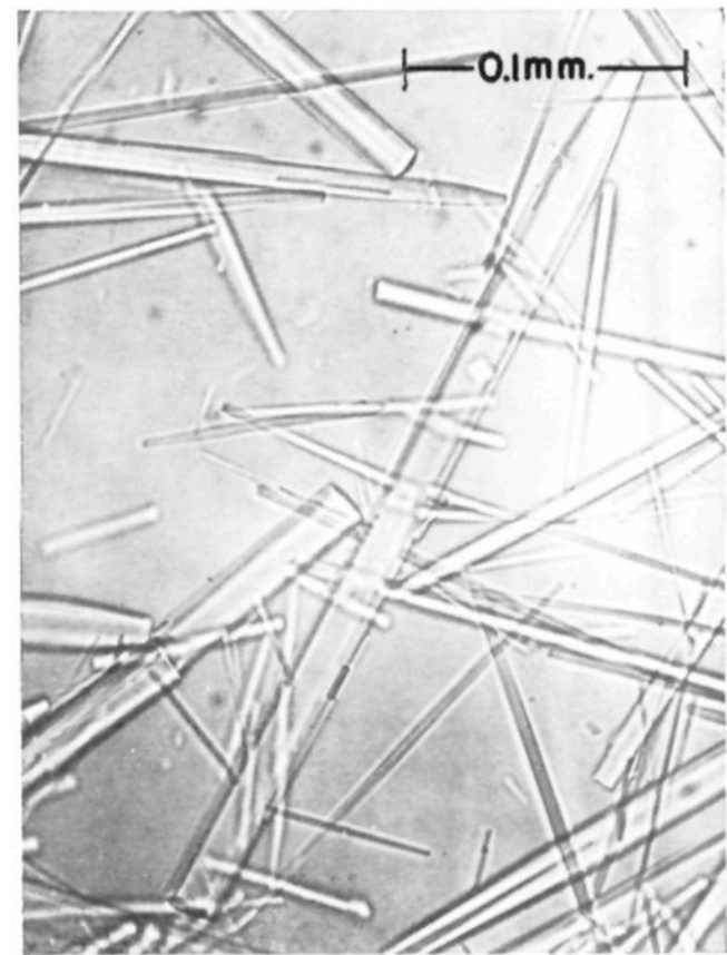
Fig. 4.—Bovine serum albumins crystallized from 0.05 mole fraction ethanol; \Gamma/2 = 0.02 ; pH 5.1; -5^\circ .
